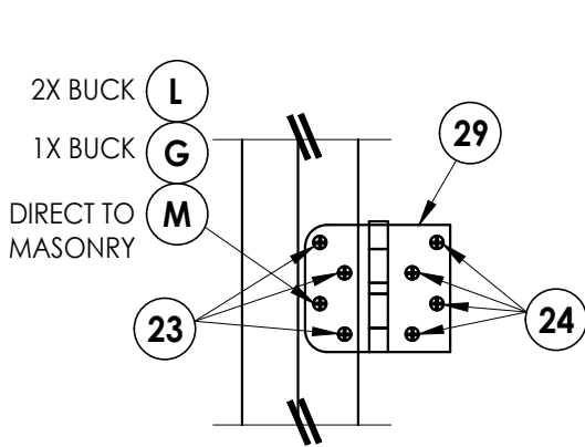
HINGE DETAIL
